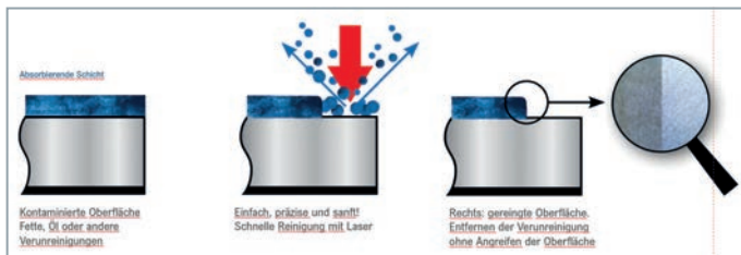
Abb. 3: General LASER treatment principal
